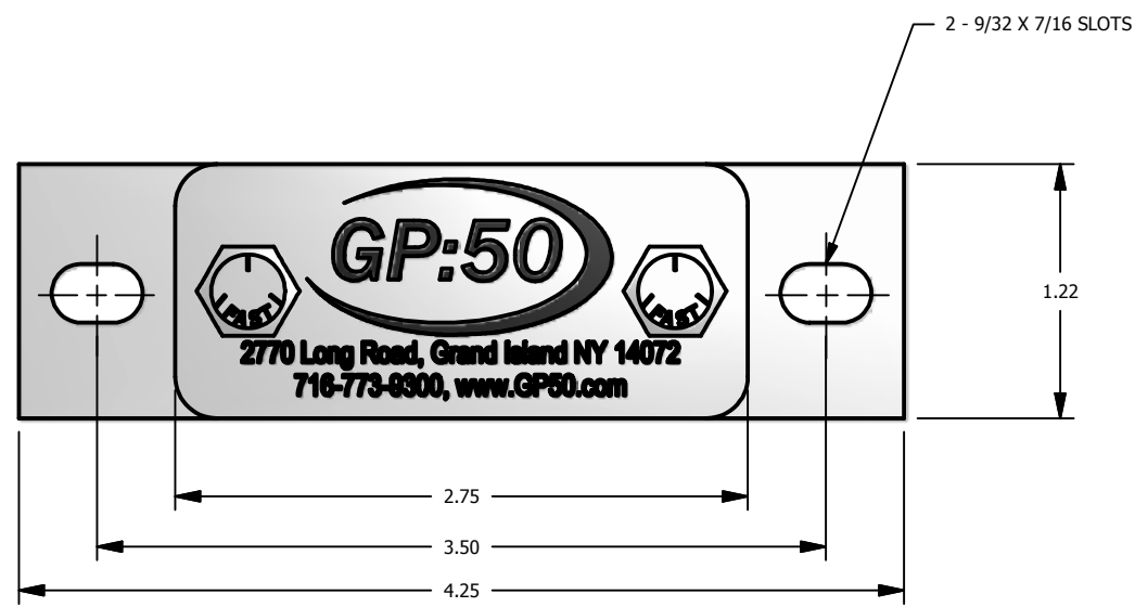
MOUNTING BRACKET DETAILS
