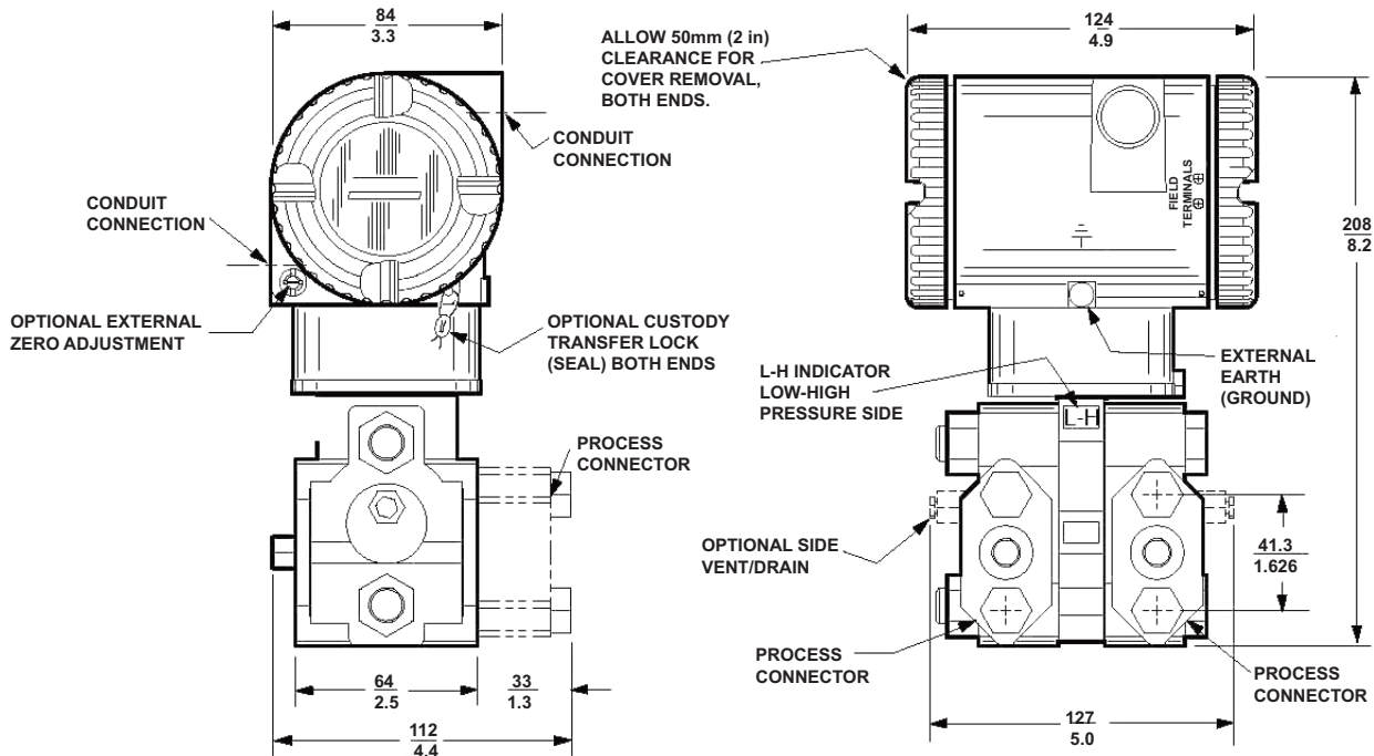
TRADITIONAL STRUCTURE DIMENSIONS (NOMINAL) \frac{mm}{in}
